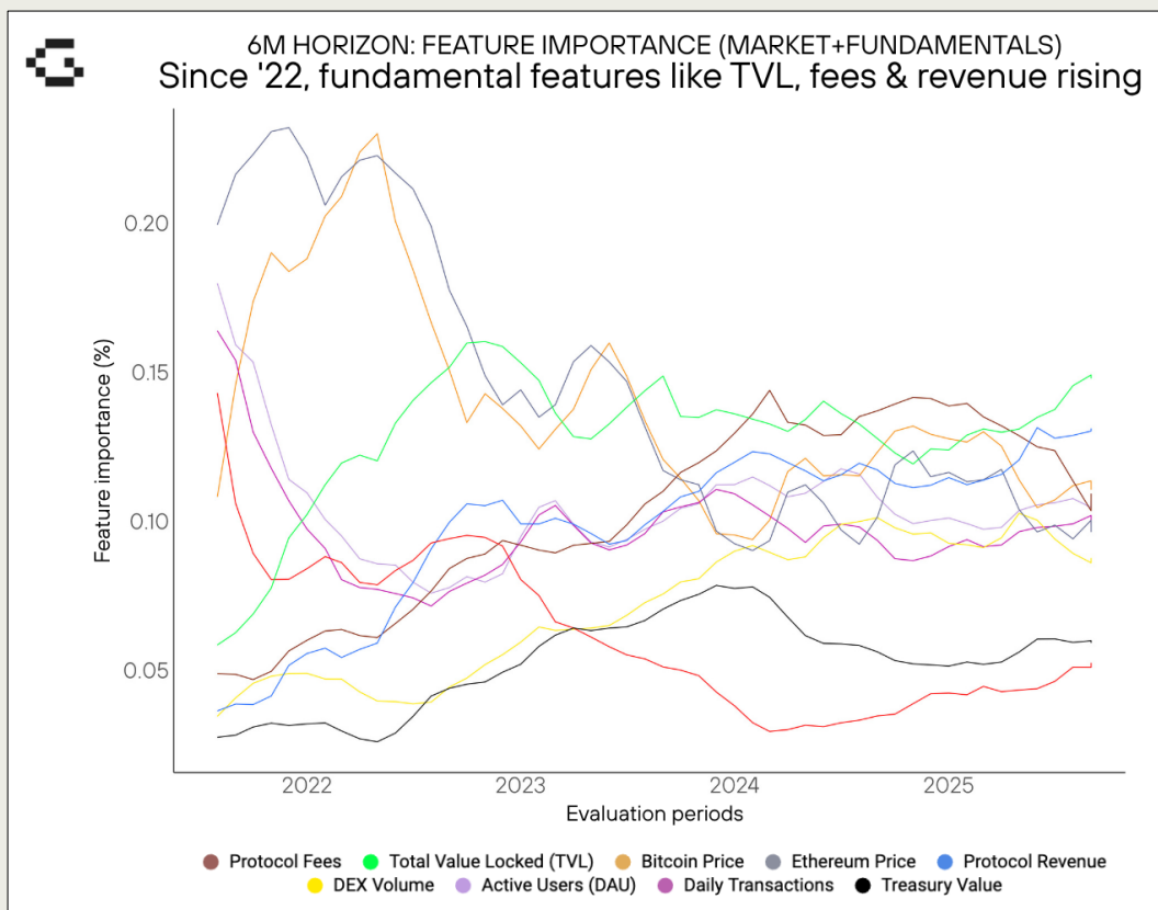
Figure 12: Feature importance trends for the 6-month horizon model. Post-2024, fundamentals dominate the mix (~74%) while BTC/ETH shrink to ~22%.
